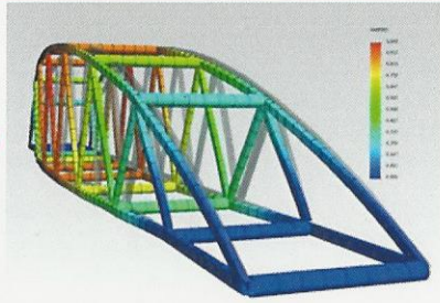
Finite Element Analysis (FEA) of space frame structures
